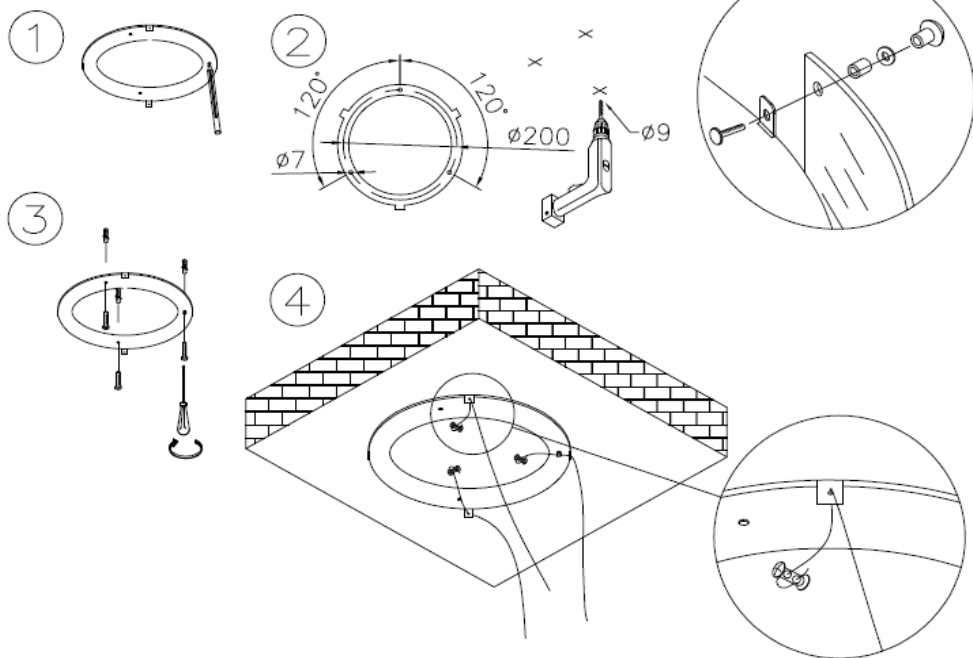
NABUCCO ISOLA FULL LED (16Kg)
